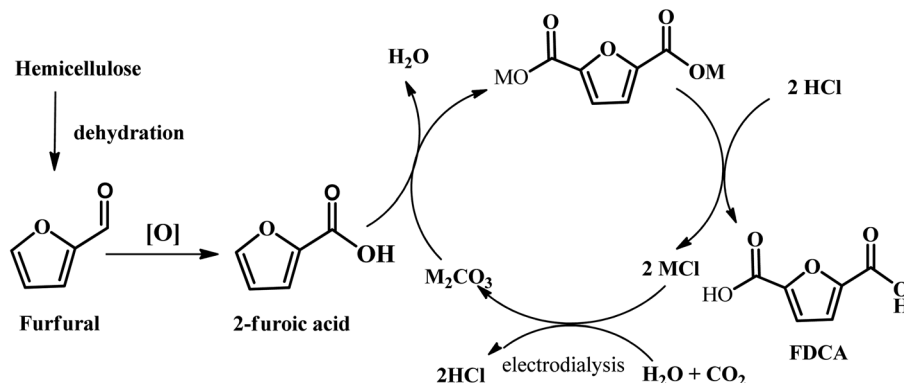
Fig. 8 Schematic illustration of the overall diagram for the production of FDCA from biomass through furfural using CO_3^{2-} -promoted C-H carboxylation. Recovery of the alkali cations is achieved by protonation of the FDCA salt and bipolar membrane electrodialysis of the resulting alkali chloride salt. Reprinted from ref. 67. Copyright 2016, The Royal Society of Chemistry.
