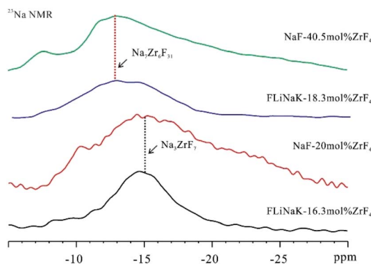
Fig. 4 ^{23}\text{Na} solid-state MAS NMR spectra of FLiNaK– \text{ZrF}_4 (16.3 mol%) and FLiNaK– \text{ZrF}_4 (18.3 mol%) eutectic solidification salt and binary salts like \text{NaF} – \text{ZrF}_4 (20 mol%) and \text{NaF} – \text{ZrF}_4 (40.5 mol%) at ambient temperature. MAS spin rate in the mentioned experiments was set to 15 kHz.
