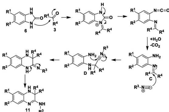
Scheme 5 Possible mechanism for the formation of dihydroquinoline 11 .
