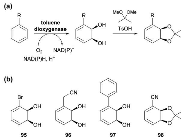
Scheme 15 Arene cis -dihydroxylation by toluene dioxygenase (TDO): (a) general reaction scheme for the dihydroxylation of a mono-substituted arene by TDO and for the conversion of the resulting diol into an acetonide. (b) Examples of commercially available arene cis -dihydrodiols or the corresponding acetonides (as of January 2021).
