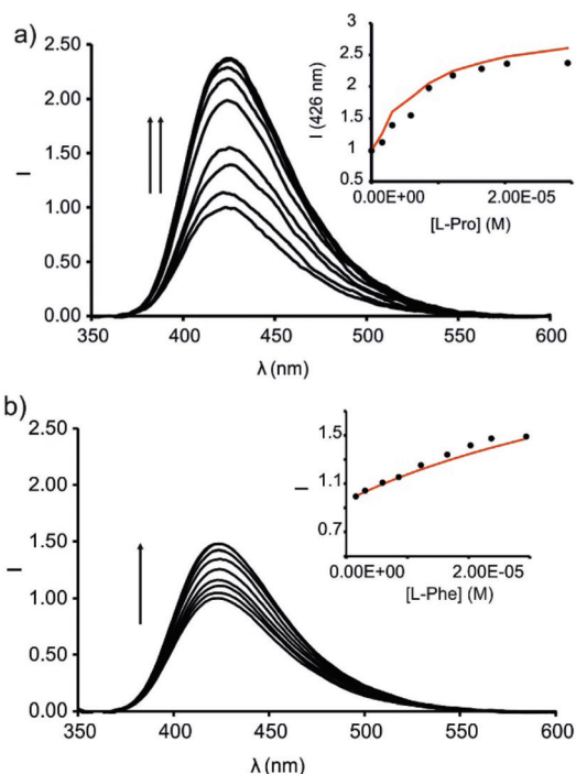
Fig. 9 Emission spectra registered during the competitive IDA experiments of 6C1in complex (1 μM) with incremental addition of L-Pro (up to 30 equiv.) (a) and L-Phe (up to 30 equiv.) (b) in dichloromethane solution; λ exc = 335 nm. Insets: plots of the emission change at 426 nm (black circles) vs. concentration of the amino acid. The red line corresponds to the fit of the titration data to a 1:1 theoretical binding model considering only two emissive species: the free cavitand and the 1:1 complex with the corresponding amino acid.
