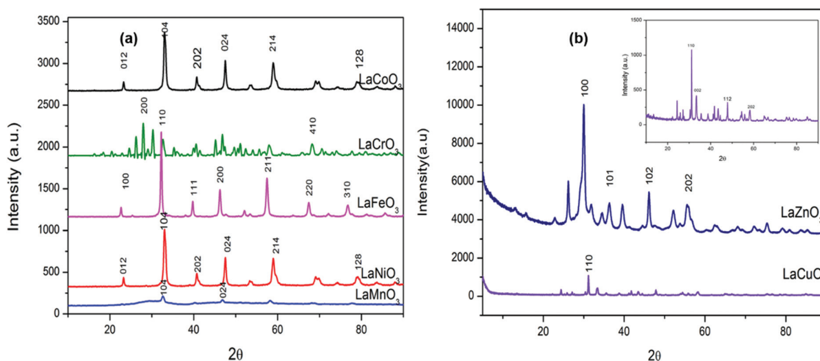
Fig. 1 Wide angle powder X-ray diffraction patterns for (a, b) \text{LaMO}_3 (M = Co, Cr, Fe, Ni, Mn, Cu, Zn) perovskites.
