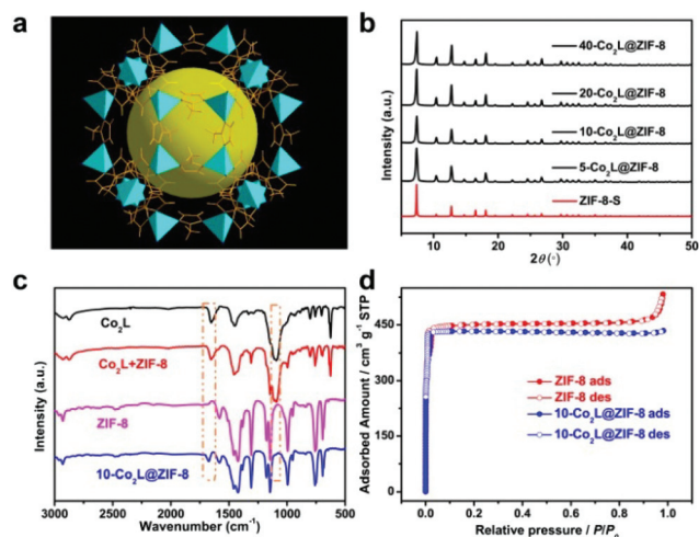
Fig. 1 (a) Cage structure of \text{Co}_2\text{L}@ZIF-8 . (b) PXRD patterns of x\text{-Co}_2\text{L}@ZIF-8 . (c) FT-IR spectra of \text{Co}_2\text{L} , \text{ZIF-8} , physically mixed \text{Co}_2\text{L} + \text{ZIF-8} , and host-guest \text{Co}_2\text{L}@ZIF-8 . (d) \text{N}_2 adsorption isotherms of \text{ZIF-8} and 10\text{-Co}_2\text{L}@ZIF-8 at 77 K.
