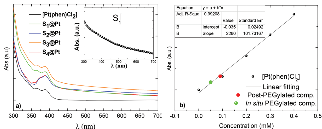
Fig. 3 (a) Absorption spectra of the composites and the Pt-complex diluted in DMSO, (inset) indicative spectrum of the primary zinc ferrite MNPs coated by propylene glycol (S 1 ) and (b) calibration curve (black circles) and amount of Pt-complex of post-PEGylated (red circle) and in situ PEGylated (green circle) composites.
