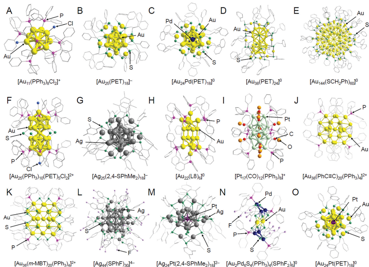
Fig. 2 Geometrical structures of atomically precise, ligand-protected metal NCs: (A) [Au 11 (PPh 3 ) 8 Cl 2 ] + , 171 (B) [Au 25 (PET) 18 ] - , 42 (C) [Au 24 Pd(PET) 18 ] 0 , 172 (D) [Au 38 (PET) 24 ] 0 , 173 (E) [Au 144 (SCH 2 Ph) 60 ] 0 , 174 (F) [Au 25 (PPh 3 ) 10 (PET) 5 Cl 2 ] 2+ , 175 (G) [Ag 25 (2,4-SPhMe 2 ) 18 ] - , 43 (H) [Au 22 (L8) 6 ] 0 , 176 (I) [Pt 17 (CO) 12 (PPh 3 ) 8 ] + , 177 (J) [Au 38 (PhC≡C) 20 (PPh 3 ) 4 ] 2+ , 178 (K) [Au 38 (m-MBT) 20 (PPh 3 ) 4 ] 2+ , 178 (L) [Ag 44 (SPhF) 30 ] 4+ , 44 (M) [Ag 24 Pt(2,4-SPhMe 2 ) 18 ] 2- , 179 (N) [Au 2 Pd 6 S 4 (PPh 3 ) 4 (SPhF 2 ) 6 ] 0 , 180 and (O) [Au 24 Pt(PET) 18 ] 0 . 26 The gray points indicate carbon atoms, and hydrogen atoms are not shown. Au 25 (SR) 18 (SR = SC12 or SG) discussed in Sections 2.1.1, 2.1.2, and 2.4 is considered to have a similar geometrical structure as [Au 25 (PET) 18 ] - (B). Au 24 Pd(SC12) 18 discussed in Section 2.1.1 is considered to have a similar geometrical structure as [Au 24 Pd(PET) 18 ] 0 (C). Au 38 (SC12) 24 discussed in Section 2.1.4 is considered to have a similar geometrical structure as [Au 38 (PET) 24 ] 0 (D). Au 144 (PET) 60 discussed in Sections 2.1.1–2.1.4 is considered to have a similar geometrical structure as [Au 144 (SCH 2 Ph) 60 ] 0 (E). These graphics were reproduced with permission from ref. 26, 42–44 and 171–180. Copyright 2016 Royal Society of Chemistry, 2008 American Chemical Society, 2015 American Chemical Society, 2013 Springer-Nature, 2014 American Chemical Society, 2016 American Chemical Society, 2010 American Chemical Society, 2018 AAAS, 2007 American Chemical Society, 2014 American Chemical Society, 2017 American Chemical Society, 2017 AAAS, 2017 American Chemical Society, 2018 Royal Society of Chemistry, respectively.
