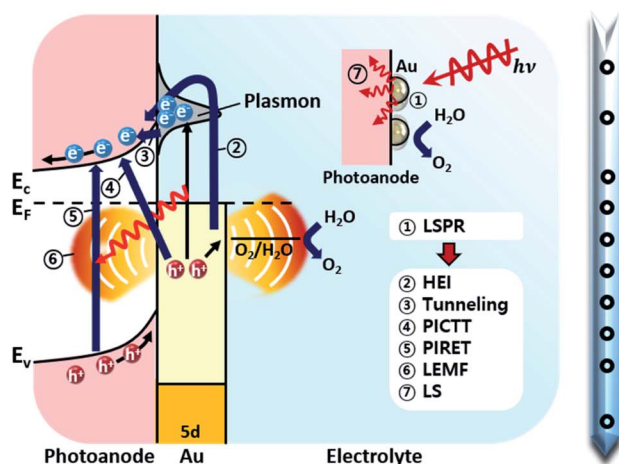
Fig. 2 (Left) Possible localized surface plasmon energy transfer mechanism from Au nanoparticles to the photoanode. Abbreviations: hot electron injection (HEI), plasmon induced metal-to-semiconductor interfacial charge transfer transition (PICTT), plasmon induced resonant energy transfer (PIRET), local electromagnetic field enhancement (LEMF), light scattering (LS). (Right) Timeline of key developments in the field of plasmon enhanced photoelectrochemical water splitting.
