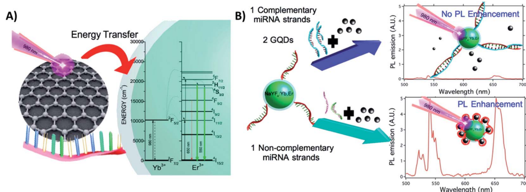
Fig. 23 UCNP-GQD sensor for miRNA detection. (A) Proposed energy-transfer mechanism between the GQDs and UCNP. (B) Schematic representation of the sensor response in the presence or absence of complementary oligonucleotides. Reprinted with permission from ref. 70. Copyright 2015, American Chemical Society.
