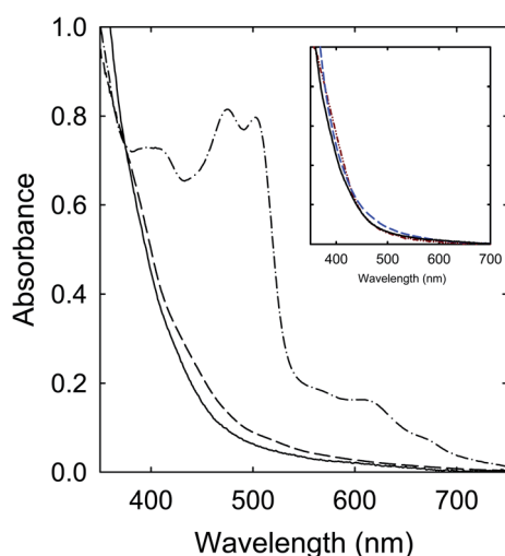
Fig. 9 Optical absorptions of samples from the CA-FA mixture processed at 160 °C for 6 h (dash-dot), 260 °C for 2 h (dashed), and 300 °C for 2 h (solid). Inset: Optical absorptions are compared between the 300 °C for 2 h sample (solid), the CA-DMF sample processed at 160 °C for 6 h (dashed), and the aqueous suspended small carbon nanoparticles (dash-dot-dot).
