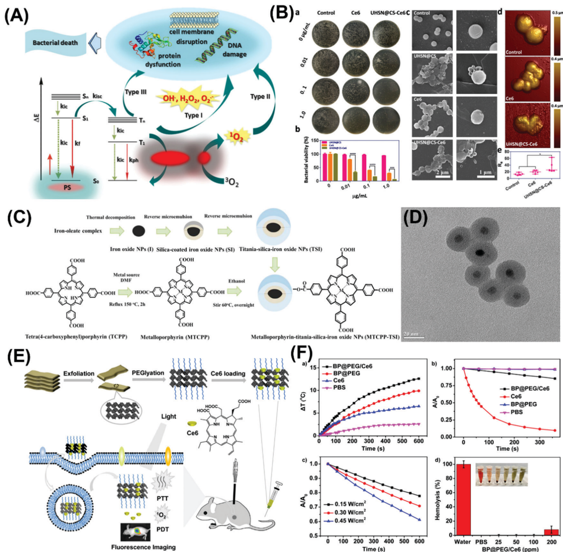
Fig. 26 Photodynamic antibacterial disinfection for dye-sensitized semiconductors. (A) Mechanism of photodynamic antibacterial therapy. Reprinted from ref. 379. (B) Photodynamic antibacterial effect of Ce6 modified with hollow \text{SiO}_2/\text{chitosan} . Reprinted from ref. 380. (C) Synthesis of \text{FeO}_x\text{-SiO}_2\text{-TiO}_2\text{-metalloporphyrins} and (D) their TEM images. (C) and (D) Reprinted from ref. 371. (E) Schematic illustration of the synthesis of BP@PEG/Ce6. (F) Photothermal evaluation and cytocompatibility (hemolysis test) of the as-prepared NPs in (E). (E) and (F) Reprinted from ref. 377.
