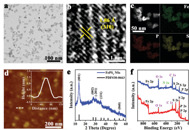
Fig. 1 (a) TEM image, (b) HRTEM image, (c) HAADF-STEM image and the corresponding EDS elemental mapping images, (d) AFM image with height profile, and (e) XRD pattern of \text{FePS}_3 NSs. (f) XPS survey spectra of \text{FePS}_3 NSs (blue) and bulk \text{FePS}_3 (red).
