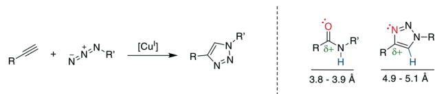
Scheme 32 Left: reaction scheme of the \text{CuI} -catalyzed azide–alkyne cycloaddition. Right: comparison of electronic and steric properties of the Z -amide and the 1,4-substituted 1,2,3-triazole. Red: H-bond acceptor position, blue: H-bond donor position.
