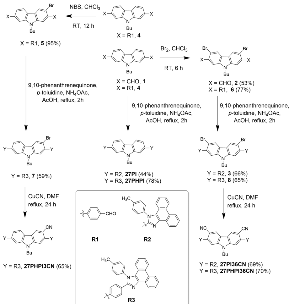
Scheme 1 Synthetic protocol of the dyes 27PI , 27PHPI , 27PI36CN , 27PHPI36CN and 27PHI36CN .
