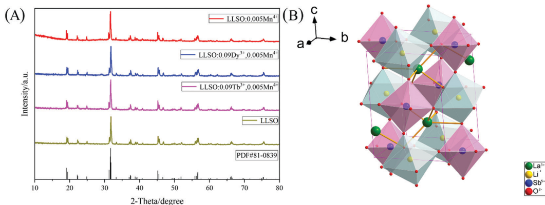
Fig. 1 (A) XRD patterns of \text{LLSO:0.005Mn}^{4+} , \text{LLSO:0.09Tb}^{3+},0.005\text{Mn}^{4+} , \text{LLSO:0.09Dy}^{3+},0.005\text{Mn}^{4+} and LLSO host. (B) Crystal structure schematic diagram of \text{La}_2\text{LiSbO}_6 .
