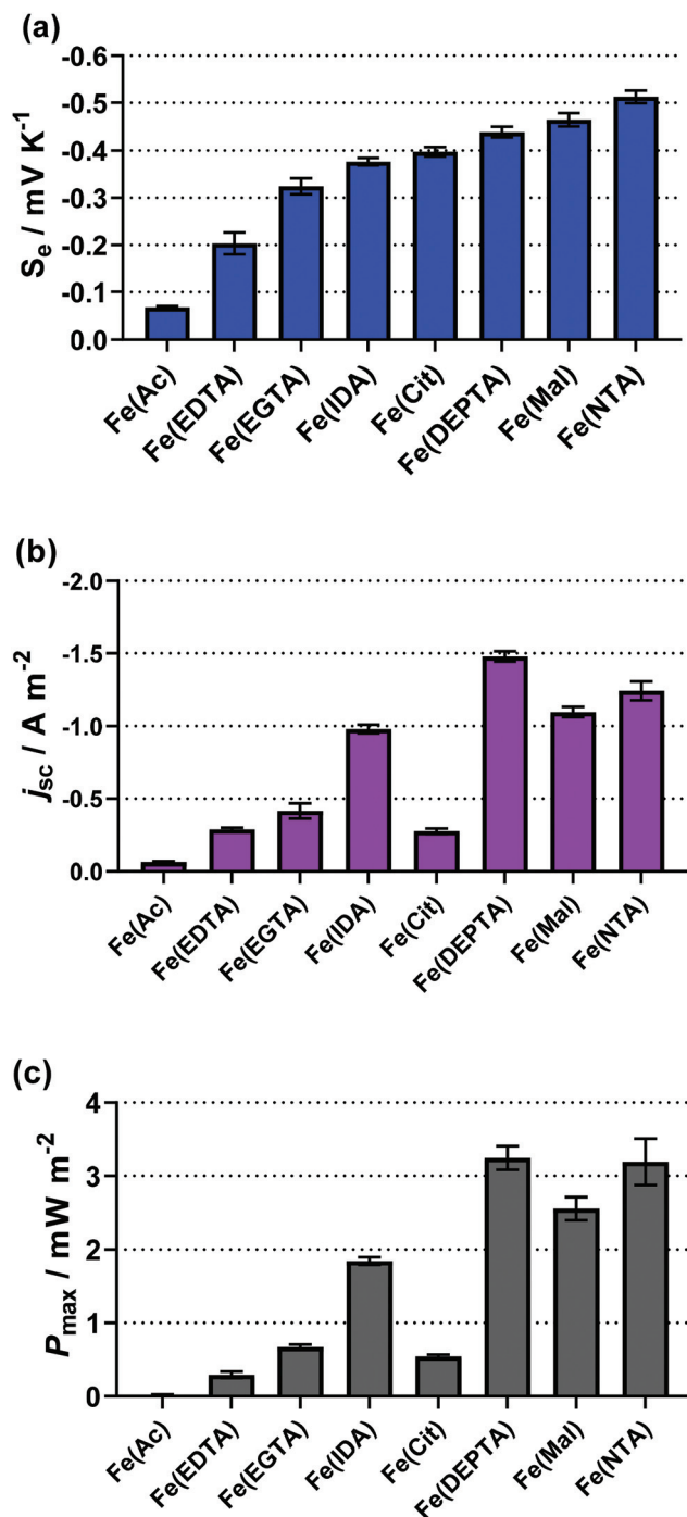
Fig. 3 Bar charts showing (a) the observed Seebeck coefficient ( S_{\text{e}} ), (b) the short-circuit current density ( j_{\text{SC}} ) and (c) the maximum power density ( P_{\text{max}} ) for the semi-optimised Fe(ligand) systems, visually displaying the values in Table 1.
