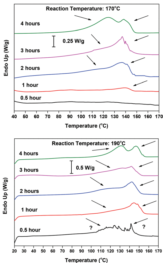
Fig. 4 DSC thermograms of the reaction samples of the esterification step, catalyzed by \text{Sb}_2\text{O}_3 at 170 °C (up) and 190 °C (down), at different reaction times.
