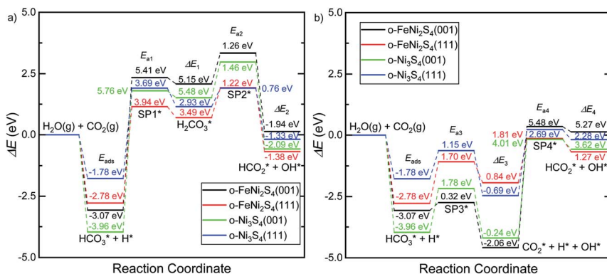
Fig. 5 Minimum energy pathways for CO 2 reduction by H 2 O via (a) substitution and (b) dissociation mechanisms on the (001) and (111) surfaces of the o -FeNi 2 S 4 and o -Ni 3 S 4 thiospinels. Minimum states and saddle points are denoted by horizontal lines linked by dashed lines. Energies are referenced to the isolated H 2 O and CO 2 molecules as well as the surface slab. Adsorbed species are denoted using the symbol *. Adsorption energies ( E_{\text{ads}} ), elemental step energies ( \Delta E_i ) and activation energies ( E_{\text{ai}} ) are also indicated.
