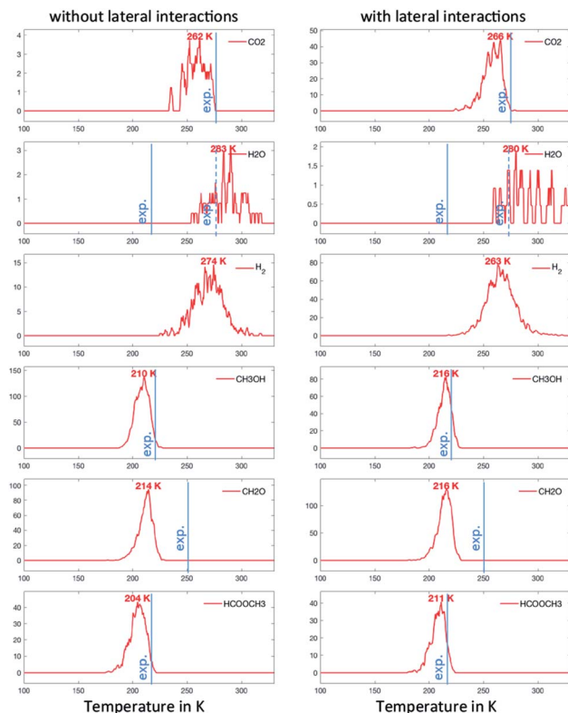
Fig. 5 TPO spectra of methanol on Au(111) for scenario #2. Temperature ramp is 10 K s -1 . The initial coverages are: 0.1 ML of CH 3 O and 0.02 ML in O.
