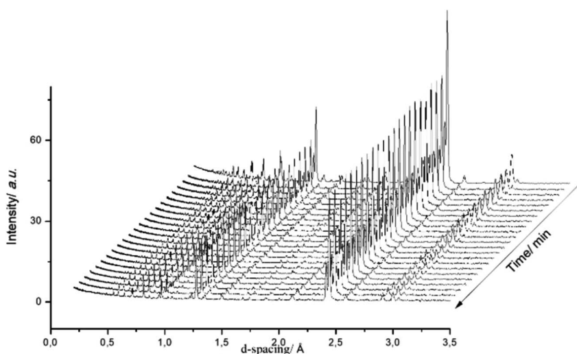
Fig. 3 Diffraction patterns of \theta - \text{Mn}_6\text{N}_{5+x} during the discharge reaction at 400 °C. In situ measurements were conducted under 60 mL min -1 75 vol% H 2 in Ar (BOC, 99.98%). Patterns were collected for 10 min.
