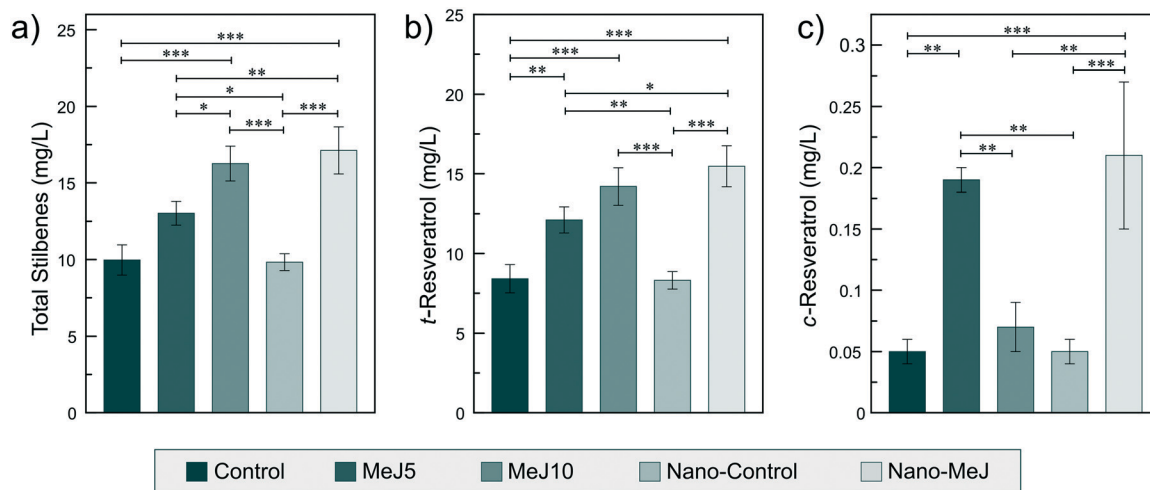
Fig. 5 Concentration (mg L -1 ) of total stilbenes (a), trans -resveratrol (b) and cis -resveratrol (c) in wines from grapes treated with water solutions containing 5 mM (MeJ5) and 10 mM (MeJ10) MeJ and 1 mM nano-MeJ. Results of grapes treated with naked nanoparticles (nano-control) and non-treated grapes (control) are also shown. Data are expressed as mean with their corresponding standard deviation as error bars. Statistically significant differences between measurements are marked with * ( P -value < 0.05), ** ( P -value < 0.01) or *** ( P -value < 0.001).
