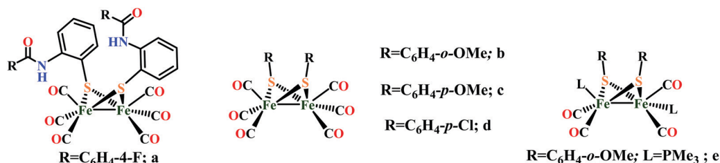
Fig. 25 Diiron model complexes with nonbridging aromatic group with all carbon atoms.
