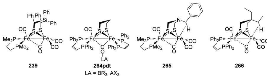
Fig. 79 Fe 2 Fe 1 models of the [2Fe-2S]-cluster exhibiting a rotated geometry.
