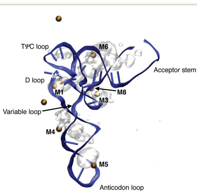
Fig. 14 Ion density around tRNA Phe of doubly charged ions Mg 2+ and Mn 2+ . Ion densities are averaged over a 1 μs simulation time and are shown together with the instantaneous geometry of tRNA Phe after 1 μs and the instantaneous position of Mg 2+ and Mn 2+ ions (ochre spheres). Ion densities are shown for an iso-value of 0.003 Å -3 . MD structure taken from ref. 80.
