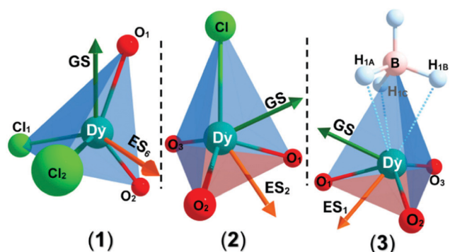
Fig. 2 Local coordination environments of 1–3 (Dy teal, Cl green, O red, B pink, H pale blue). Arrows represent CASSCF-SO calculated magnetic axis ( g_z vector), GS (dark green), and selected ES (orange) with significant angles of deviation of the g_z vector from the GS.
