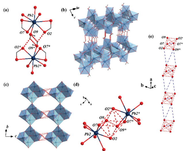
Fig. 3 (a) View of the hydrogen bonds of O9–H···O2 and O9*–H···O9 in MFM-722(Pb)-H 2 O. (b) View of the layers of [Pb 4 O 18 ] ∞ stabilised via inter-layer hydrogen bonding in MFM-722(Pb)-H 2 O. The linker is omitted for clarity. (c) Potential pathways for proton transfer in MFM-722(Pb)-H 2 O along the a axis. The linker is omitted for clarity. (d) View of the [O6] supra-octahedron. (e) Continuous hydrogen bonding pathway consisting of the [O6] supra-octahedra viewed along the a axis. Pb: dark blue; O: red; C: grey; N: blue; Pb–O polyhedra: light blue; hydrogen bond: dash red lines.
