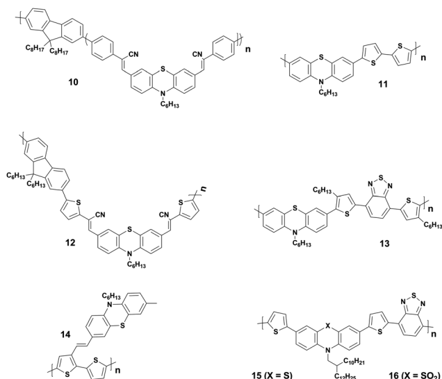
Fig. 6 Phenthiazine (PTZ)-based polymeric donor materials. The key properties of OSCs employing these dyes in the BHJ blend are listed in Table 1.
