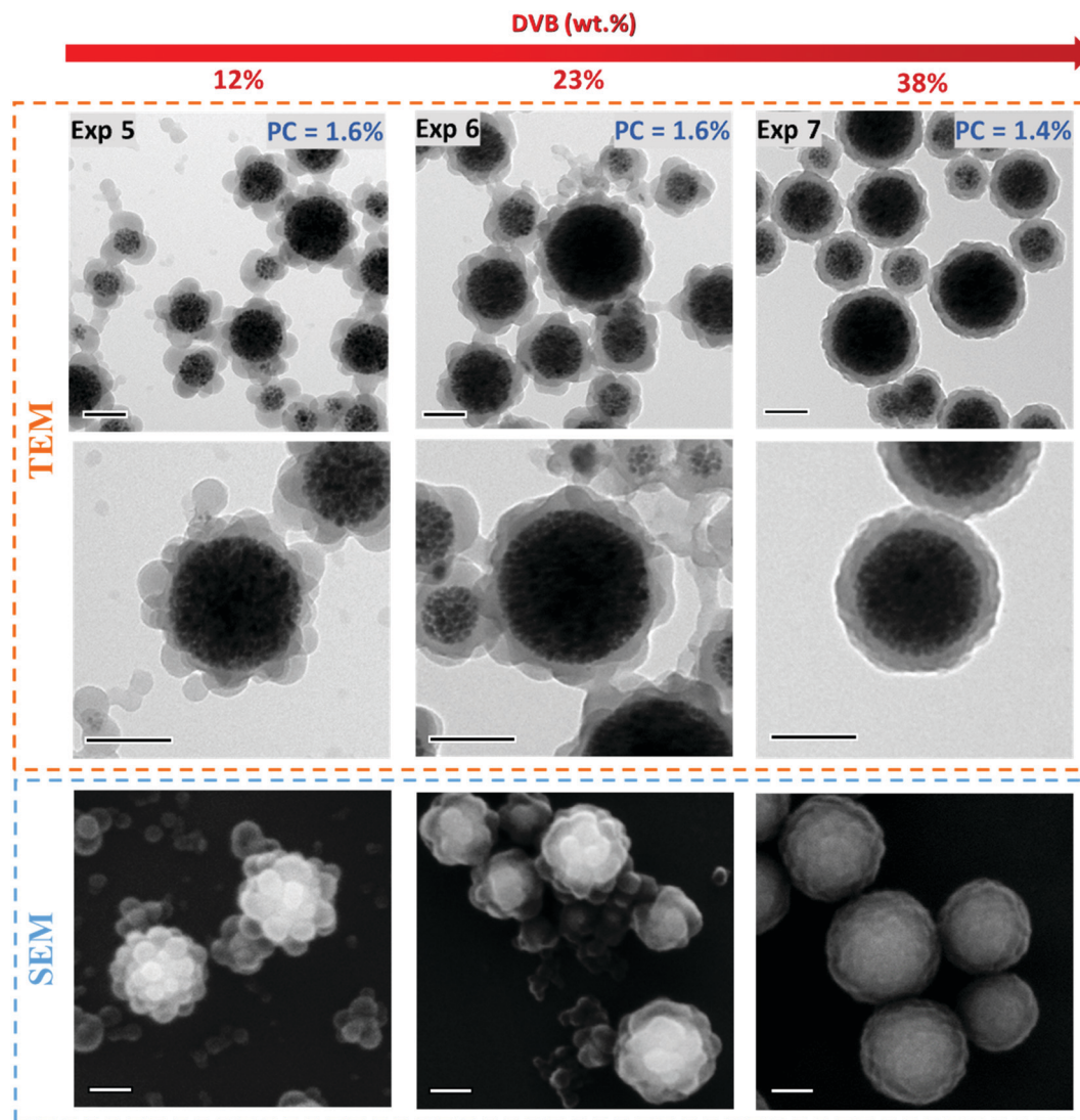
Fig. 5 TEM and SEM micrographs of PDMAEMA@MLPs synthesized by seeded semi-batch emulsion polymerization of styrene ( PC_{theo} = 2.5\% ) in the presence of increasing amounts of DVB: 12 wt% and 23 wt% (based on overall monomer mass) (Exp. 5, 6 and 7, respectively, Table 1), introduced either in the initial load or in both the initial load and the feed (see Table S3, ESI† for detailed experimental conditions). Scale bar: 100 nm. Additional micrographs are presented in the ESI.†
