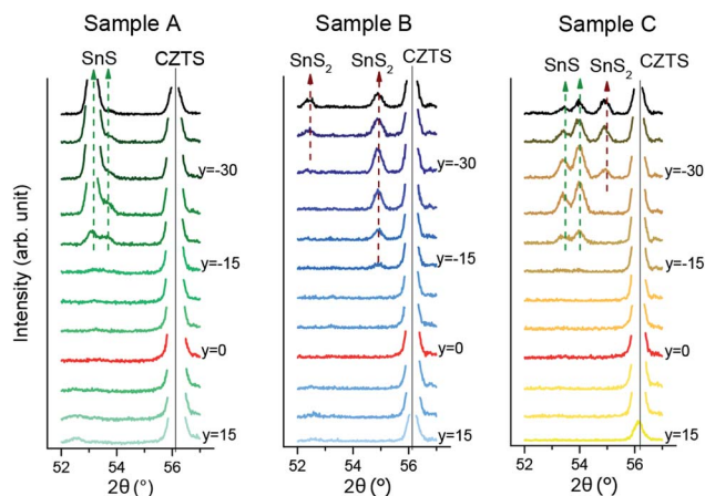
Fig. 4 XRD patterns of samples A, B and C in a 2\theta range with expected SnS and \text{SnS}_2 reflections. y denotes the distance to the \text{Cu/Sn} = 2 line in mm.
