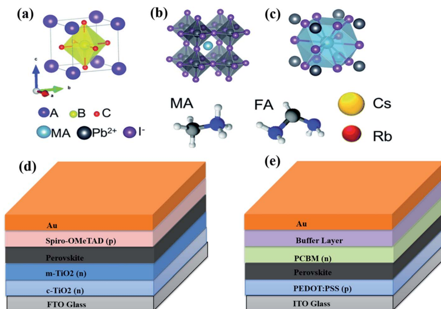
Fig. 1 (a) Unit cell of a general cubic perovskite. (b) MAPbI 3 illustrating the octahedral coordination around the lead ions. (c) MAPbI 3 illustrating the cuboctahedral coordination around the organic ion. Reproduced by permission ref. 11, Copyright 2017 Royal Society of Chemistry. (d) n–i–p and (e) p–i–n perovskite solar cell device architectures.
