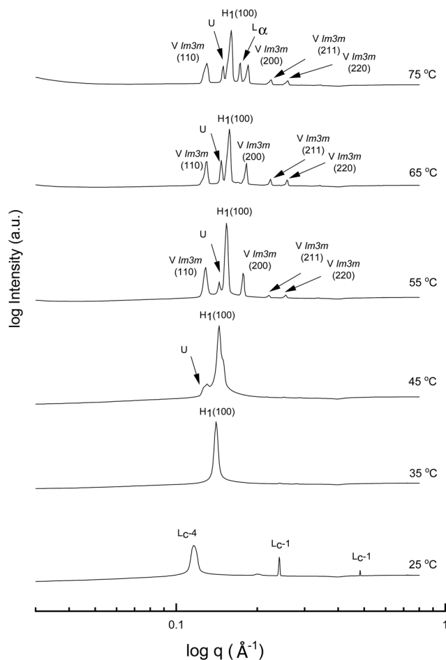
Fig. 3 SAXS patterns of 70 wt% CTAB in water at temperatures from 25 to 75 °C. The liquid crystal phases are denoted as normal hexagonal ( H_1 ), normal primitive cubic ( V_1 ( Im\bar{3}m )), lamellar ( L_c ), and unassigned transient (U) liquid crystal phases. The symbols L_c -1 and L_c -4 denote lamellar surfactant crystalline phases.
