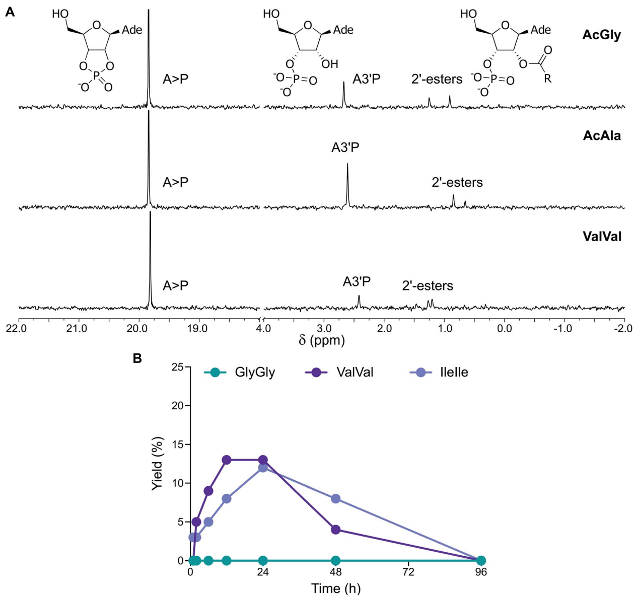
Fig. 5 Simultaneous activation of nucleotides and peptides in the presence of vesicles made of prebiotic fatty acids. (A) ^{31}\text{P} -NMR spectra showing the activation of \text{A}3'\text{P} in the presence of AcGly, AcAla and ValVal and DA : DOH : DHO (4 : 1 : 1 ratio) vesicles after 12 h in DCI buffer, pH 6. (B) Plot reporting the formation and the hydrolysis of 2'-esters of \text{A}3'\text{P} under activation conditions in the presence of the dipeptides GlyGly, ValVal or Ilelle and DA : DOH : DHO (4 : 1 : 1 ratio) vesicles in DCI buffer, pH 6.
