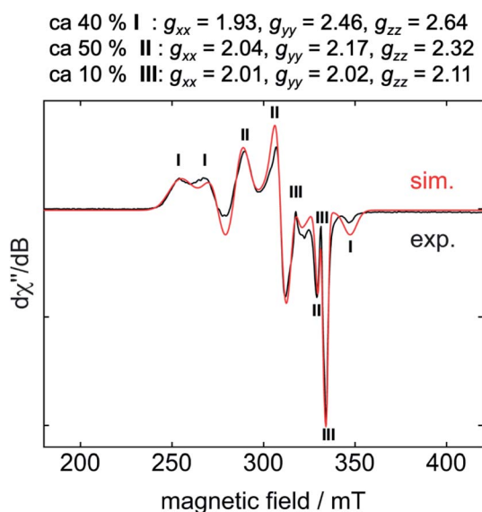
Fig. 2 EPR spectrum ( -203\text{ }^{\circ}\text{C} ) of the reaction mixture of 1 with \text{C}_6\text{F}_6 after 5 s at -78\text{ }^{\circ}\text{C} in thf.
