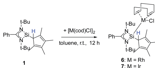
Scheme 6 Synthesis of \{[\text{PhC}(\text{NtBu})_2]_2(\text{C}_5\text{Me}_4\text{H})\text{Si}\{\text{RhCl}(\text{cod})\}\} ( 6 ) and \{[\text{PhC}(\text{NtBu})_2]_2(\text{C}_5\text{Me}_4\text{H})\text{Si}\{\text{IrCl}(\text{cod})\}\} ( 7 ).
