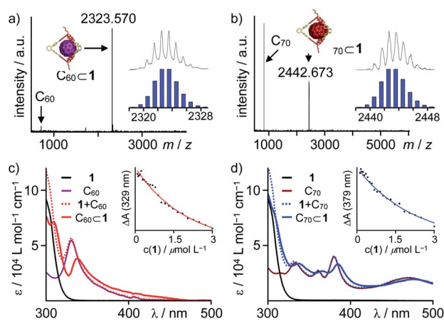
Fig. 2 MALDI-TOF MS (TCNQ, CHCl 3 ) for 1 : 1 mixtures of 1 and (a) C 60 and (b) C 70 (insets show comparison of measured and simulated isotope patterns); UV/Vis titration experiments for complex formation between 1 and (c) C 60 (black 1 , purple C 60 , dotted red 1 + C 60 , red C 60 ⊂ 1 derived from global fit to 1 : 1 model, inset shows fit to 1 : 1 model at \lambda = 329 \text{ nm} ) and (d) C 70 (black 1 , brown C 70 , dotted blue 1 + C 70 , blue C 70 ⊂ 1 derived from global fit to 1 : 1 model, inset shows fit to 1 : 1 model at \lambda = 379 \text{ nm} ).
