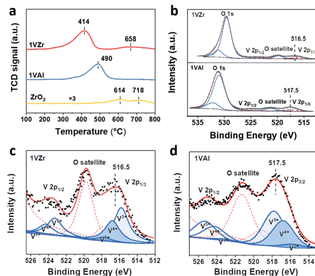
Fig. 4 (a) \text{H}_2 -TPR profiles of 1VZr, 1VAL and pure \text{ZrO}_2 . (b) XPS O 1s and V 2p peaks for 1VZr and 1VAL. Deconvolution results of V 2p 3/2 for (c) 1VZr and (d) 1VAL after reduction for 30 minutes.
