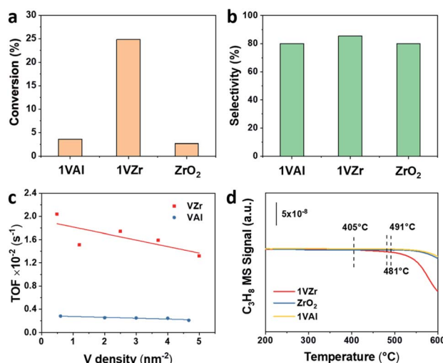
Fig. 2 (a) Initial propane conversion and (b) propylene selectivity (based on all products) of 1VAl, 1VZr and ZrO 2 . Reaction conditions: m_{\text{cat}} = 0.4 g; C 3 H 8 : N 2 : H 2 = 7 : 36 : 7; T = 550 °C; inlet flow = 50 mL min -1 . (c) Comparison of TOF values between VZr and VAl with different V densities. (d) C 3 H 8 -TPSR of 1VZr, ZrO 2 and 1VAl.
