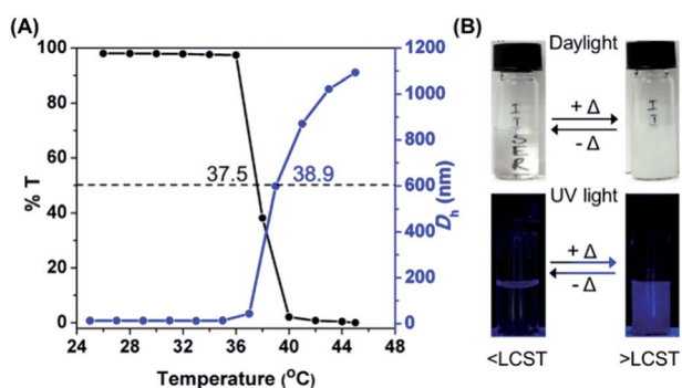
Fig. 3 (A) Variation of %T and D_h of a 0.1 wt% aqueous PNVCCL solution as a function of temperature. (B) Photographs of the same PNVCCL solution acquired under daylight and UV irradiation (365 nm) below and above the LCST.
