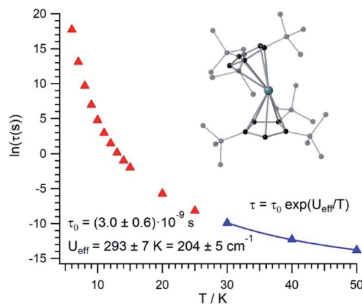
Fig. 3 [\text{U}(\text{Cp}^{\text{ttt}})_2]^+ thermal evolution of the Orbach-based relaxation time \tau , along with fit to determine both the Orbach prefactor \tau_0 and the effective barrier U_{\text{eff}} in the thermally activated regime ( T \geq 30 K).
