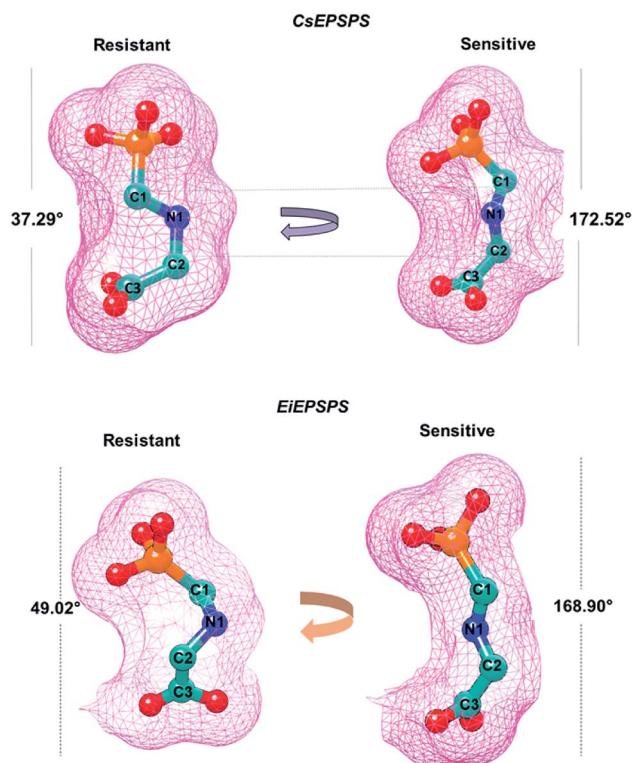
Fig. 3 Average values of the dihedral angles assumed by glyphosate when complexed with resistant and sensitive Conyza sumatrensis 5-enolpyruvyl shikimate-3-phosphate synthase ( CseEPSPS ) and Eleusine indica EPSPS ( EieEPSPS ) structures. The dihedral angle values were obtained over 100 ns of molecular dynamics simulation for sensitive and resistant variants of both species.
