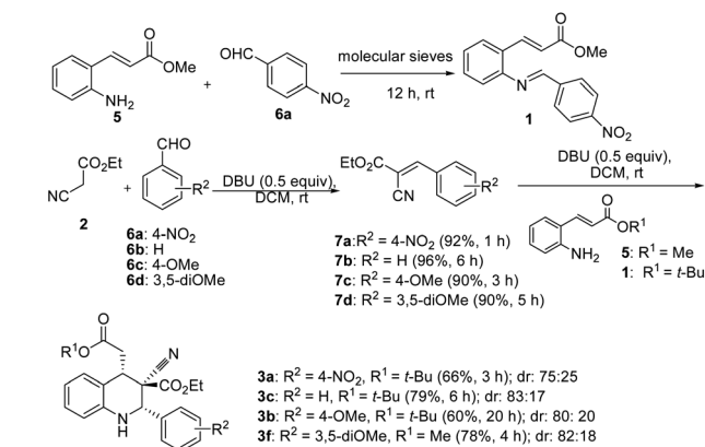
Scheme 2 Two component approach via Knoevenagel intermediate.
