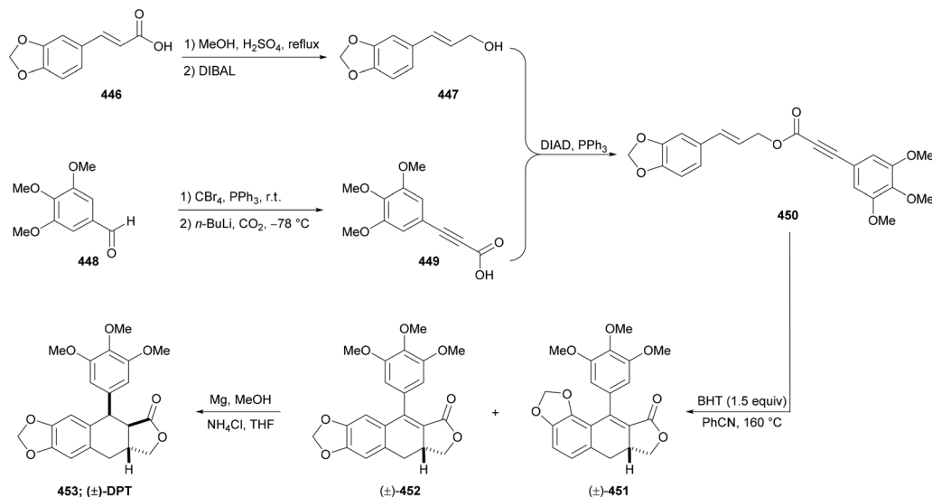
Scheme 109 Synthesis of deoxy podophyllotoxin by the ISDA strategy.
