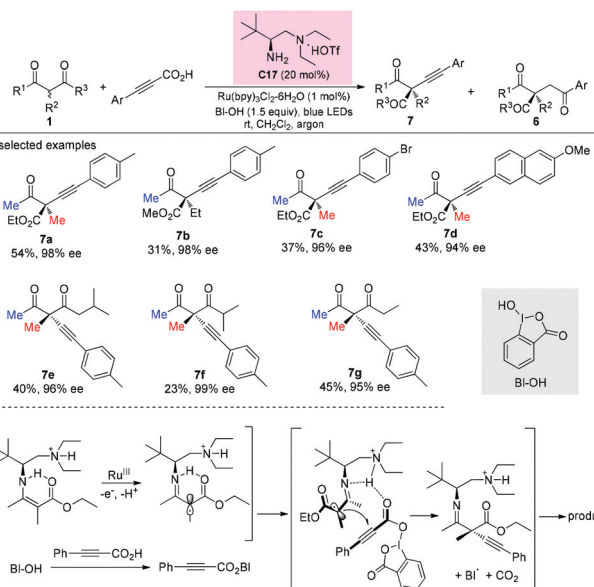
Scheme 48 Asymmetric alkylation via primary amine-photocatalysis.
