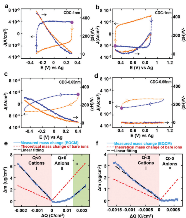
Fig. 8 CV and EQCM frequency response of (a and b) CDC-1 nm and (c and d) CDC-0.65 nm (e and f) in 2 M EMI-TFSI/AN below (a and c) and above (b and d) the immersion potential (the purple dot is where the cycle starts; orange and blue curves indicate charge and discharge of ions, respectively). Electrode mass change vs. charge during the polarization of (e) CDC-1 nm and (f) CDC-0.65 nm in 2 M EMI-TFSI + AN (blue solid lines are measured mass change (EQCM); red dashed lines are the theoretical mass change of neat ions calculated from Faraday's law and the black dashed line shows the linear fitting of measured mass change). Reproduced with permission from ref. 46. Copyright 2014 American Chemical Society.
