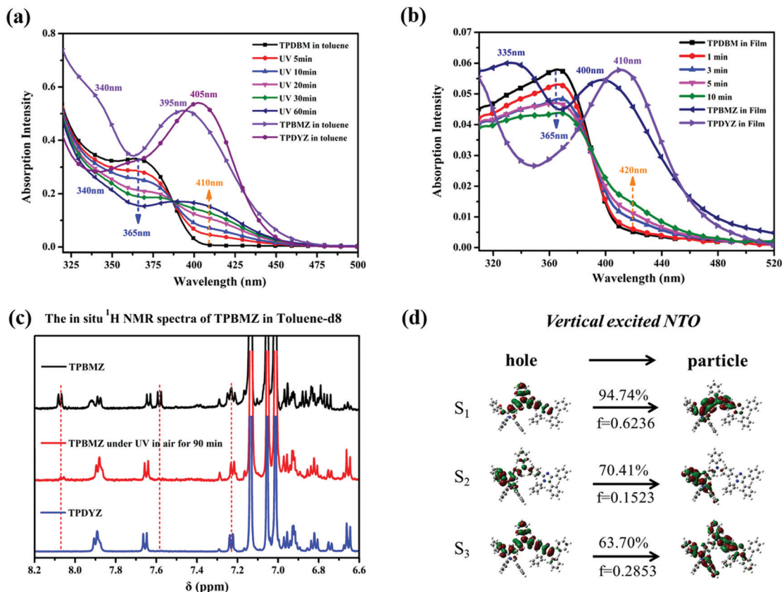
Fig. 6 In situ UV spectra of TPDBM (a) in toluene solution and (b) as a film. (c) In situ ^1\text{H} NMR spectra of TPBMZ. (d) The natural transition orbital (NTO) distributions of TPBMZ relating to S_0 \rightarrow S_1 , S_0 \rightarrow S_2 and S_0 \rightarrow S_3 excitations at the TD-OB97X/6-31G(d,p) level using S_0 state geometry.
