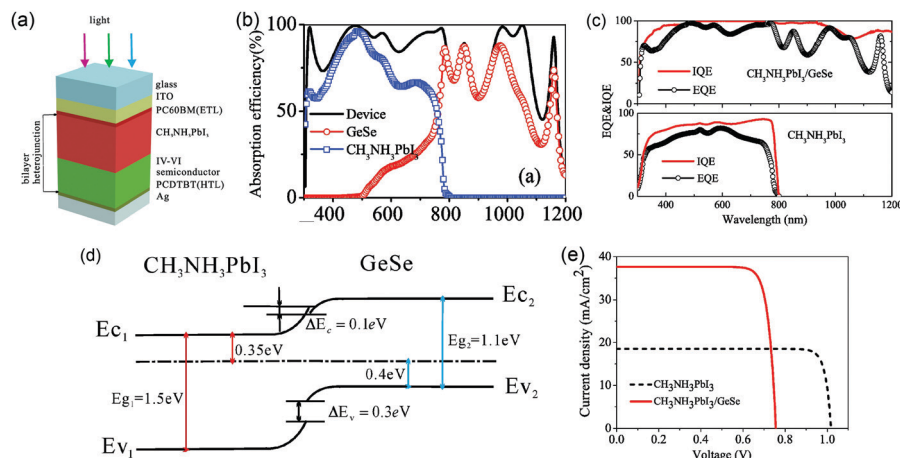
Fig. 8 (a) Schematic structure of the \text{CH}_3\text{NH}_3\text{PbI}_3/\text{GeSe} bilayer solar cell. (b) The calculated absorption spectrum for the device of the bilayer solar cell. (c) External quantum efficiency and internal quantum efficiency of the \text{CH}_3\text{NH}_3\text{PbI}_3/\text{GeSe} bilayer solar cell and \text{CH}_3\text{NH}_3\text{PbI}_3 solar cell. (d) The band alignment of the \text{CH}_3\text{NH}_3\text{PbI}_3/\text{GeSe} bilayer. (e) Current density–voltage ( J – V ) curves of the \text{CH}_3\text{NH}_3\text{PbI}_3/\text{GeSe} bilayer solar cell and \text{CH}_3\text{NH}_3\text{PbI}_3 solar cell. Reprinted with permission from ref. 93. Copyright 2017, Elsevier.
