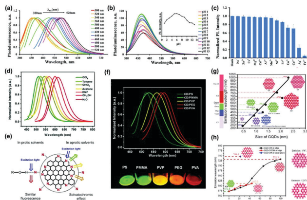
Fig. 5 (a) The excitation-dependent normalized PL for NS-CDs via a one-step facile microwave-assisted pyrolysis using citric acid and thiourea, (b) pH-dependent PL spectra at different pH values, (c) the normalized PL intensity of NS-CDs in different metal ions. 88 (Reprinted with permission from the Royal Society of Chemistry, Copyright 2019.) (d) The effect of solvents on the PL of CDs prepared from p -phenylenediamine excited by 420 nm light. (e) The emission processes of the CDs in different solvents. (f) PL spectra of five CDs/polymer films (excited at 420 nm). 89 (Reprinted with permission from the Royal Society of Chemistry, Copyright 2017.) (g) Calculated emission wavelength (nm) of the diameter of GQDs using the time-dependent density-functional theory (TDDFT) method. The solid line is the linear fit of zigzag-edged GQDs. (h) Emission wavelength versus oxidized GQDs attached –OH and –COOH groups to edge carbon atoms. (coverage of –OH and –COOH groups from 0 to 100%). 90 (Reprinted with permission from the Royal Society of Chemistry, Copyright 2014.)
