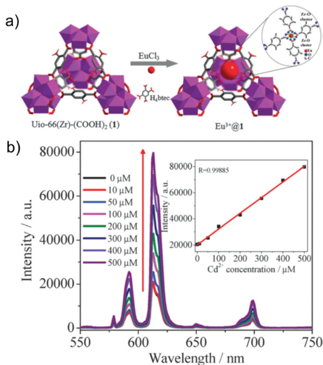
Fig. 8 (a) Synthetic representative structure of \text{Eu}^{3+}@MOF . (b) Fluorescence intensity change of \text{Eu}^{3+}@1 upon the addition of \text{Cd}^{2+} ions (inset: linear relationship of the fluorescence intensity of the probe enhanced by \text{Cd}^{2+} ions). Reproduced with permission from ref. 84. Copyright 2015, Royal Society of Chemistry.
