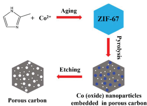
Fig. 1 Schematic illustration of the synthetic route for MOF-derived carbon using ZIF-67 as an example.
